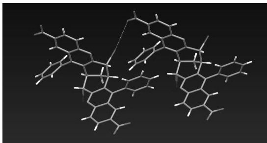
FIGURE 4 Two molecules of 4 with same chirality interact via Br O with a distance of 3.45 Å.
