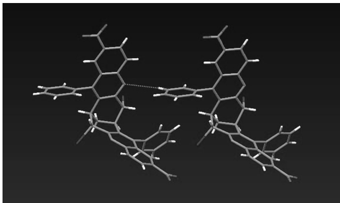
FIGURE 2 Part of the crystal structure of 4 showing two molecules of 4 interacting together. Color code: C = gray, N = blue, H = white, O = red, and Br = dark red.
