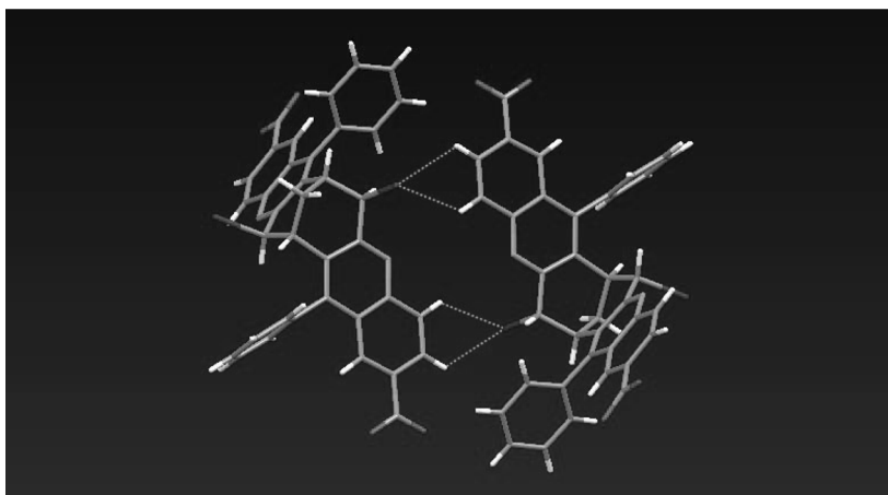
FIGURE 3 Centrosymmetric double \text{Br}\cdots\text{H}\cdots\text{C}\cdots\text{Ar} hydrogen interaction between opposite enantiomers of 4 with \text{C}\cdots\text{H}\cdots\text{Br} distances of 3.22 and 3.05 Å in each motif. Color code: C = gray, N = blue, H = white, O = red, and Br = dark red.
